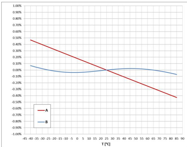
Characteristic of the dependence of the measurement error on temperature for R_0=47k\Omega (A – X1, B – X2)
